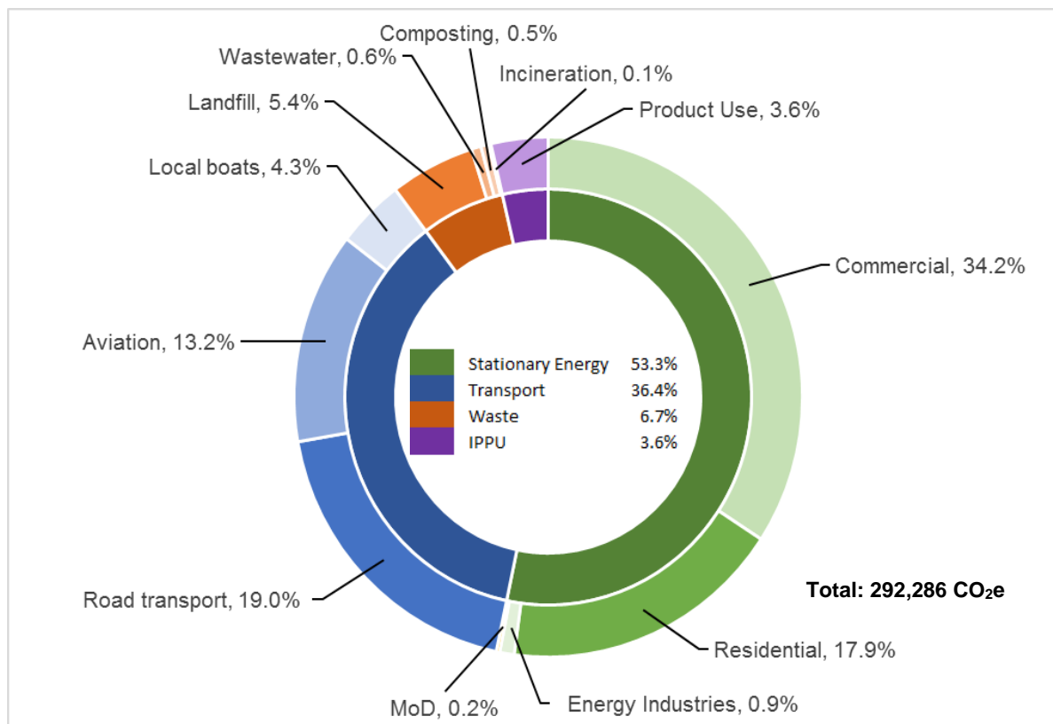
Figure 3: Gibraltar's 2017 'manageable' emissions
