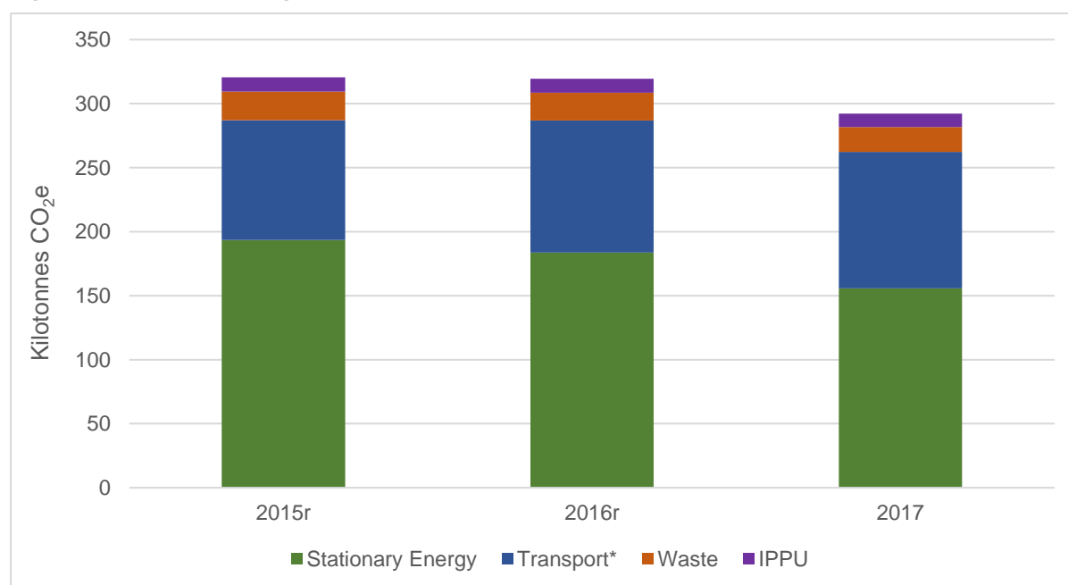
Figure 4: Gibraltar's 'manageable' emissions for 2015r, 2016r and 2017
