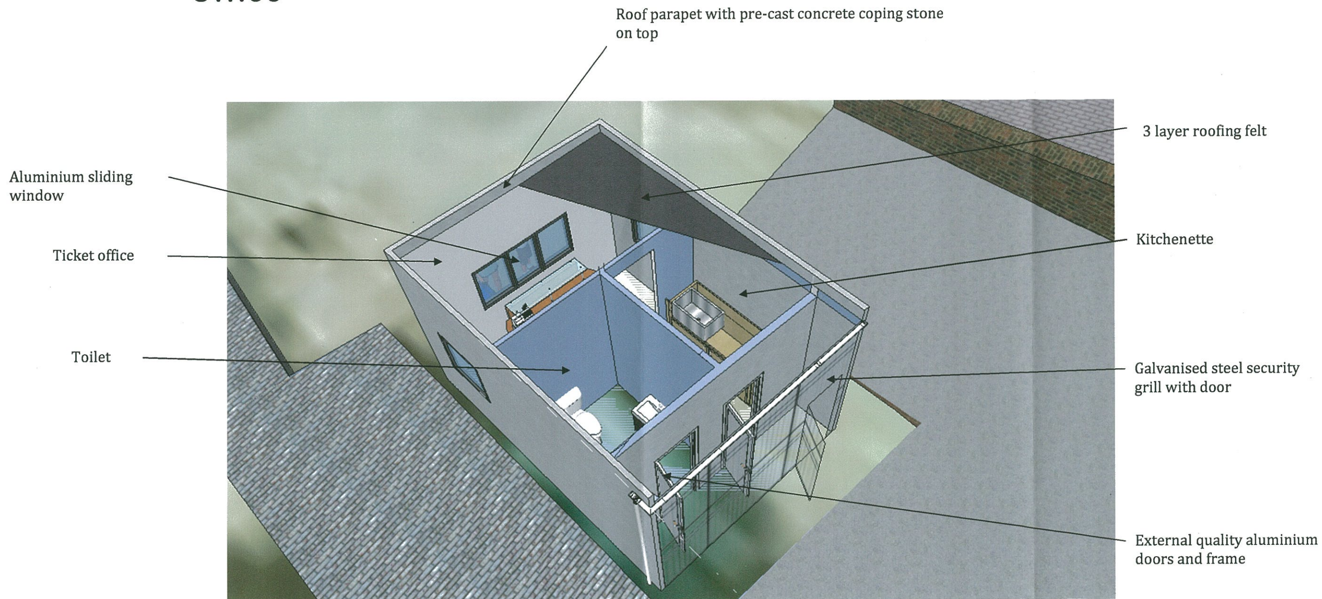
PROPOSED PERSPECTIVE ISOMETRIC VIEW
