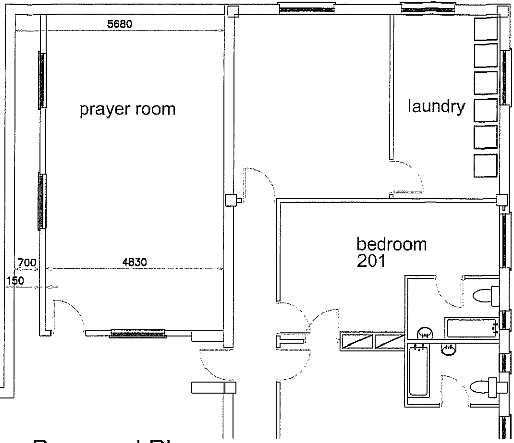
Proposed Plan
