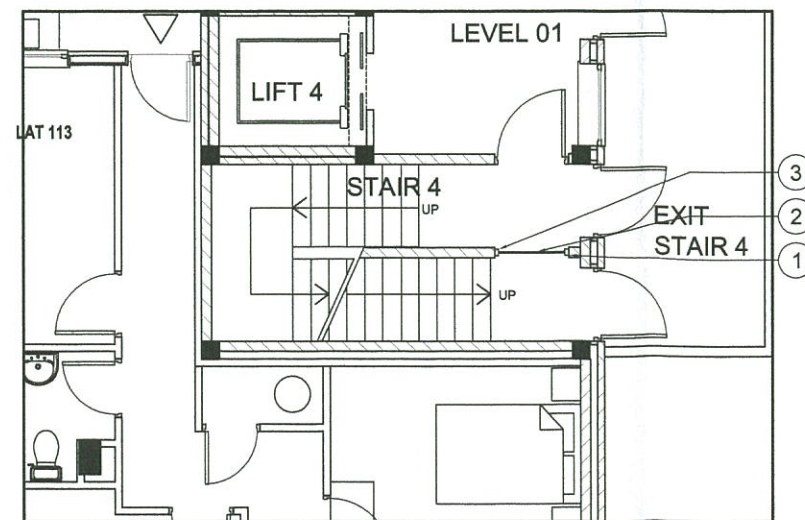
2 - STAIRCORE 4 - PROPOSED PLAN - 1:50@A1
