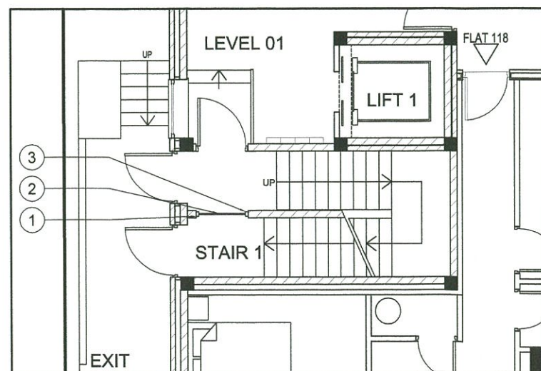
1 - STAIRCORE 1 - PROPOSED PLAN 1:50@A1
