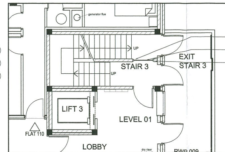
3 - STAIRCORE 3 - PROPOSED PLAN 1:50@A1
