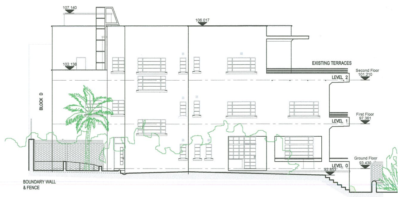
WEST ELEVATION
