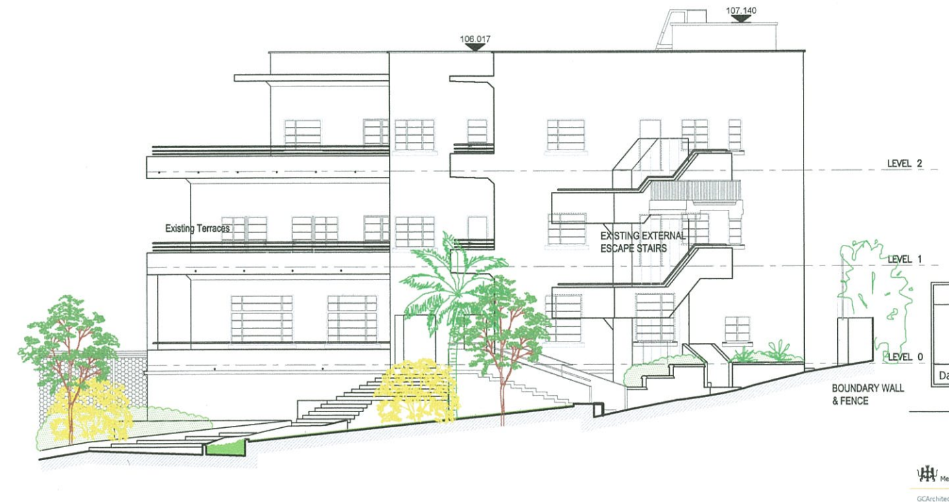
EAST ELEVATION
