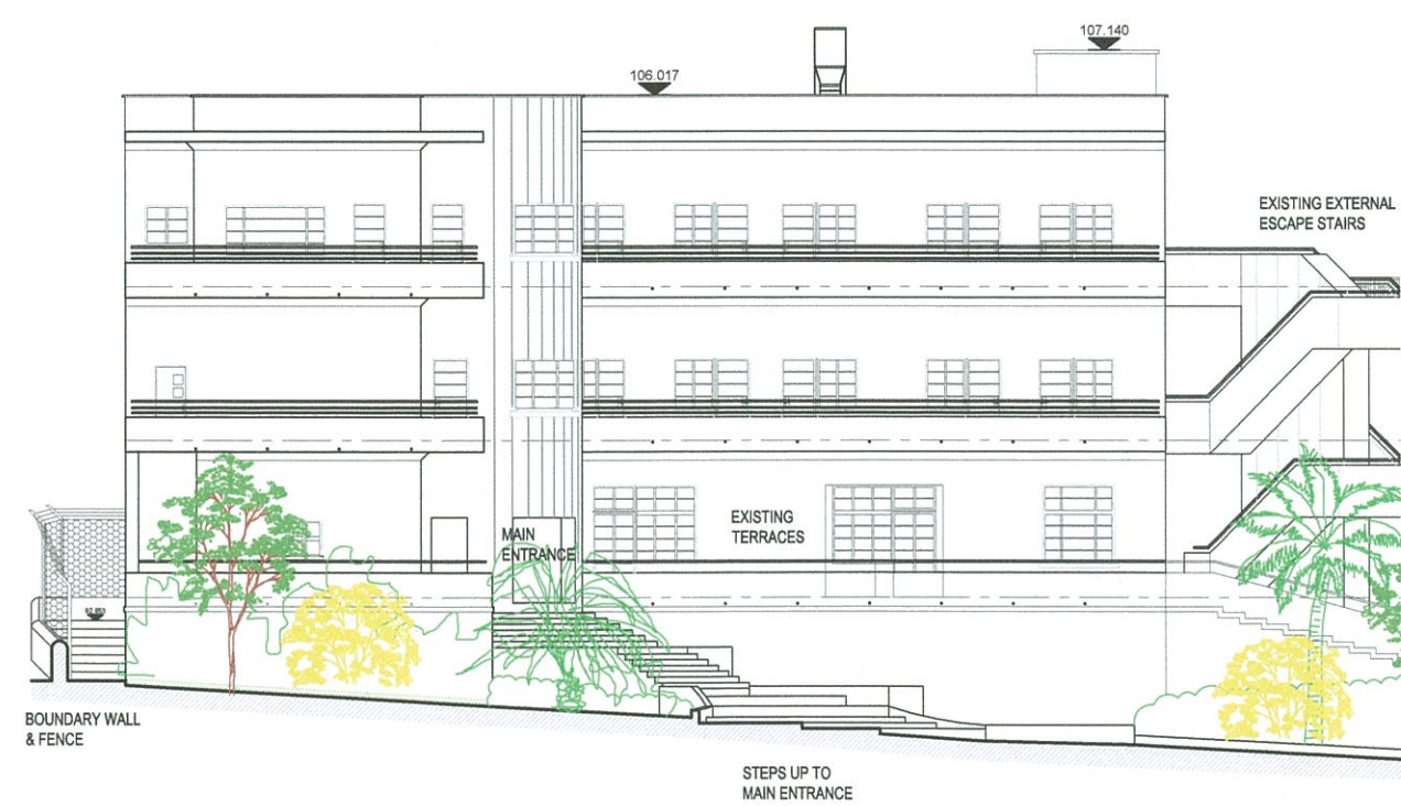
SOUTH ELEVATION
