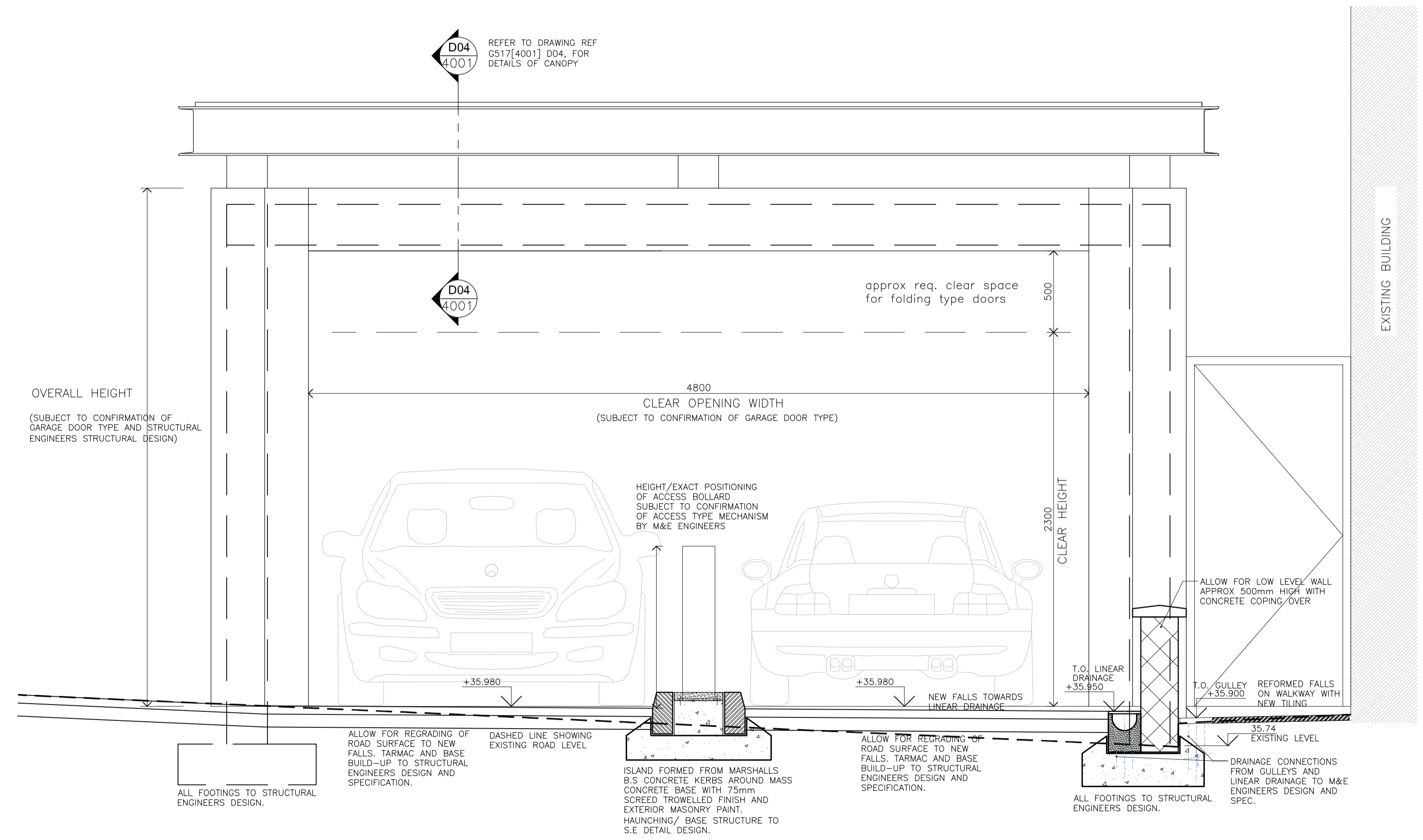
D01[4002] CAR PARK ENTRANCE ELEVATION + DETAILS SCALE 1:20
