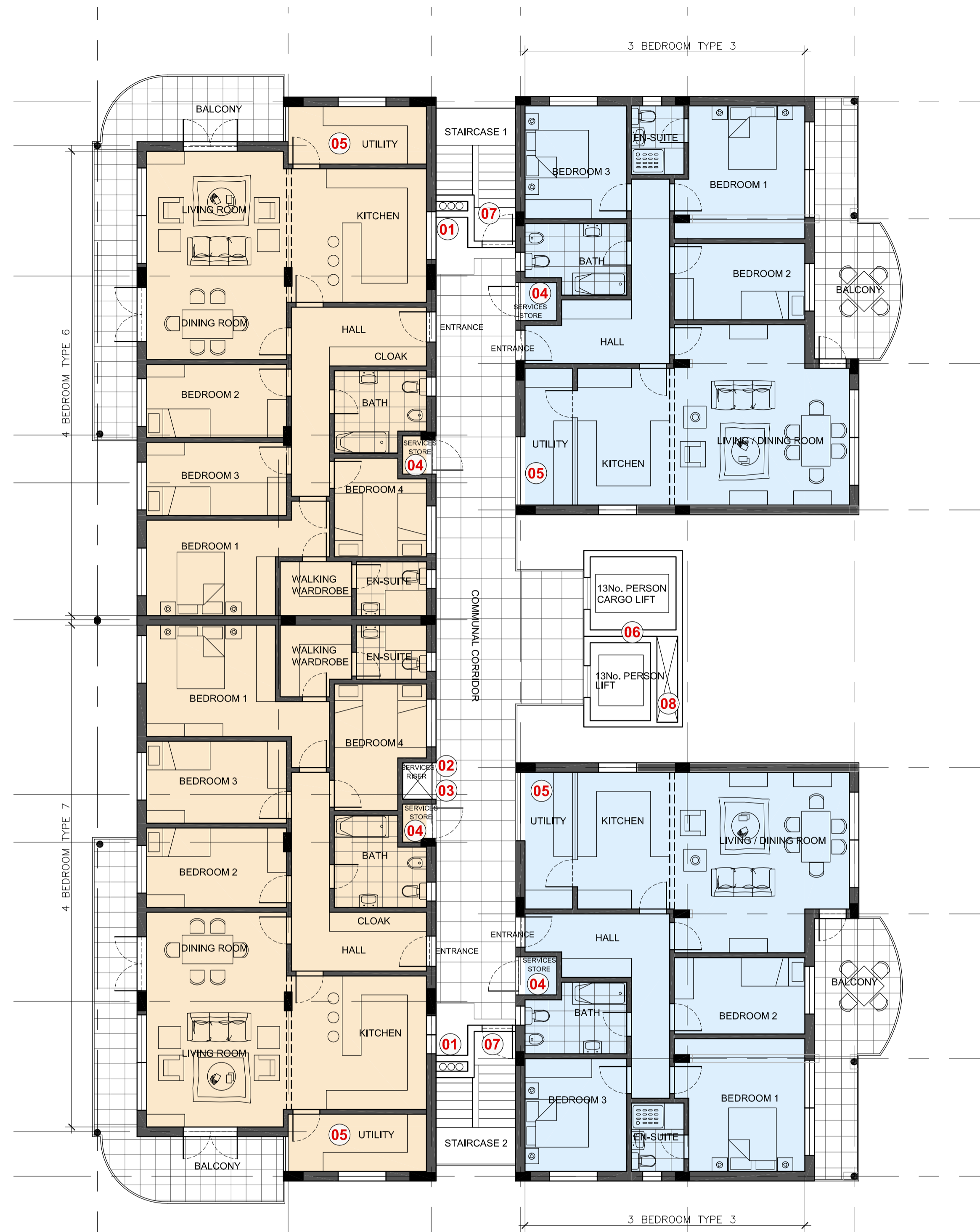
BLOCK 2 & 3 - 14TH FLOOR LEVEL PENTHOUSE FLATS Scale 1/100
