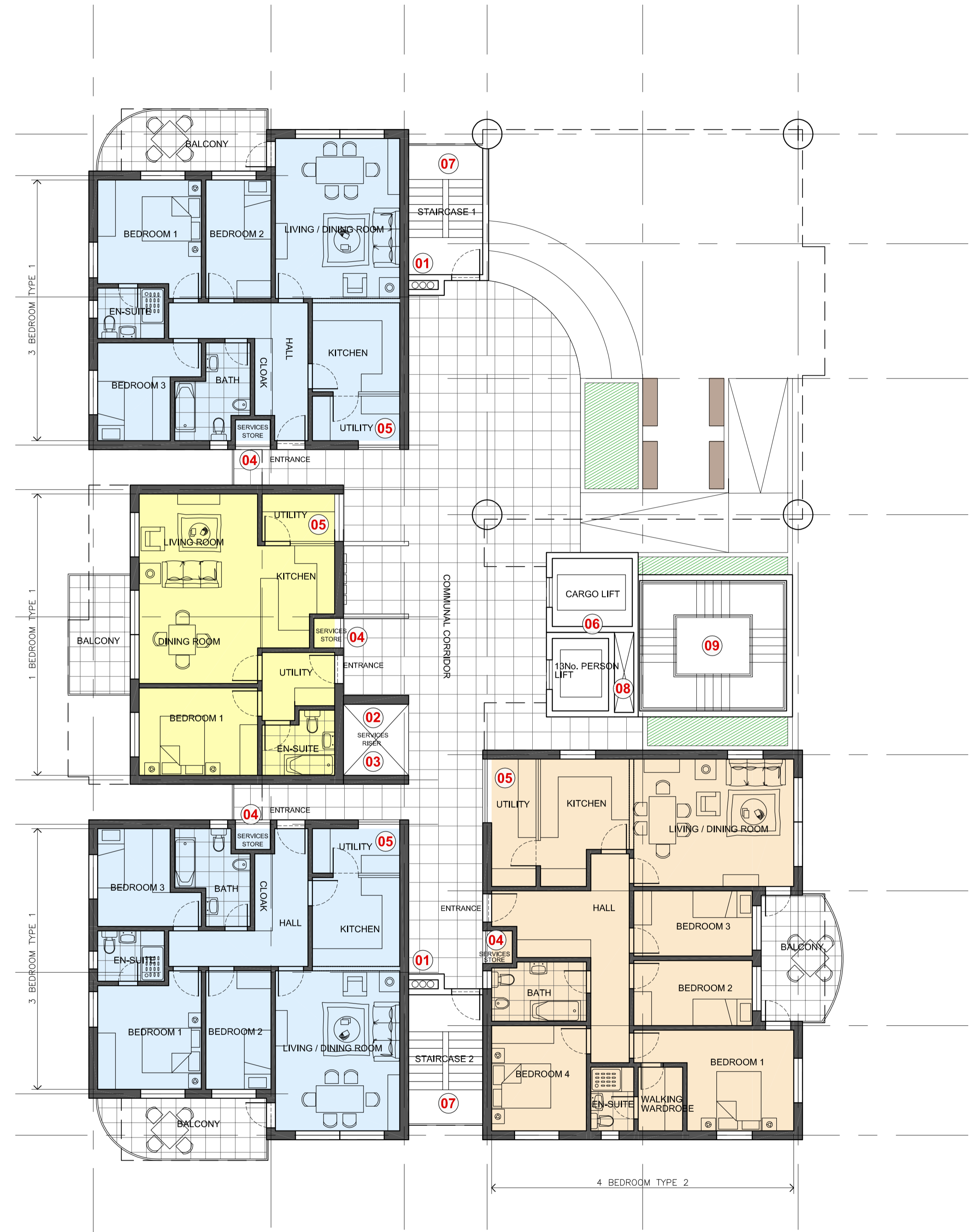
BLOCK 2 - 3RD FLOOR PODIUM LEVEL FLATS Scale 1/100
