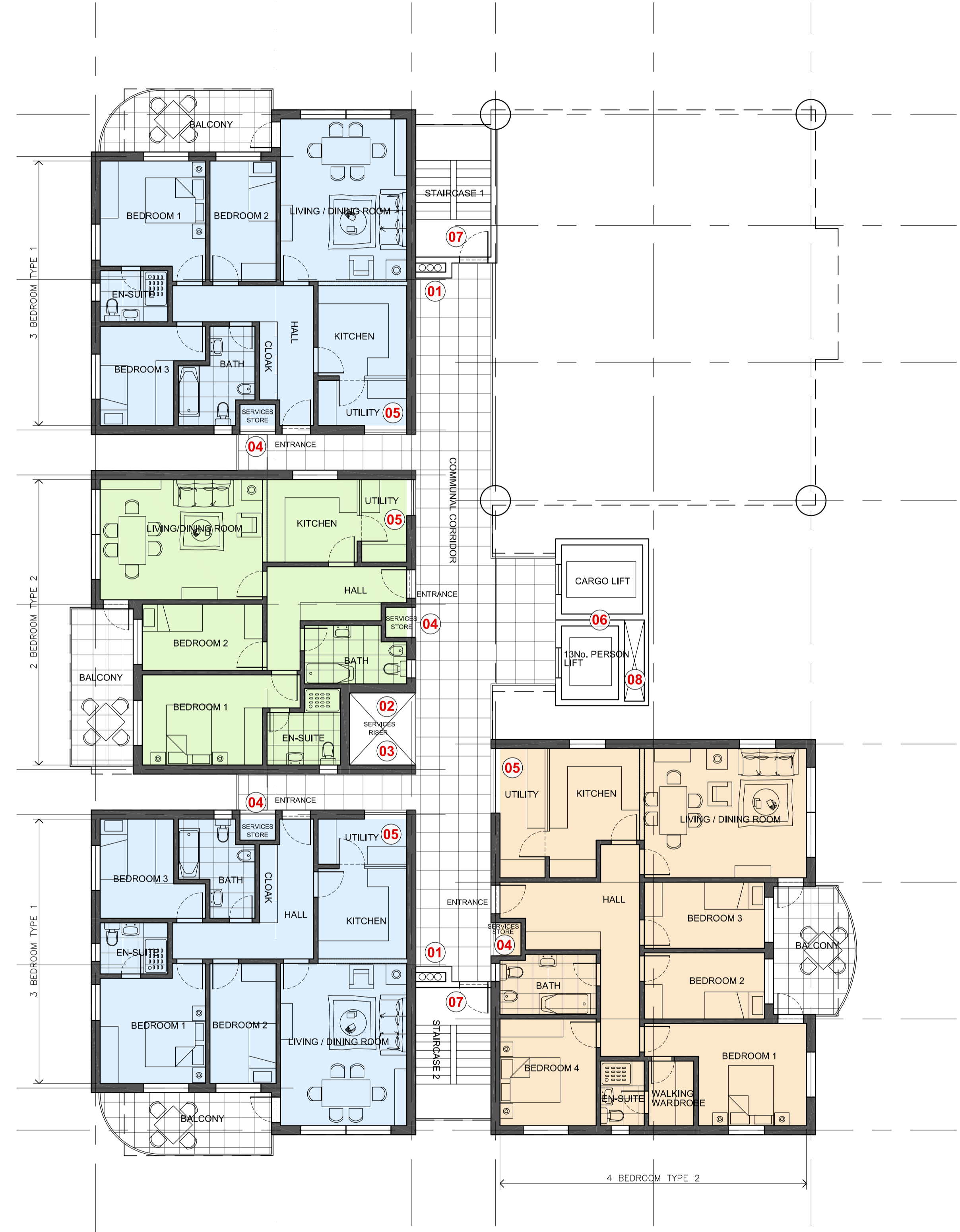
BLOCK 2 - 4TH FLOOR LEVEL FLATS Scale 1/100
